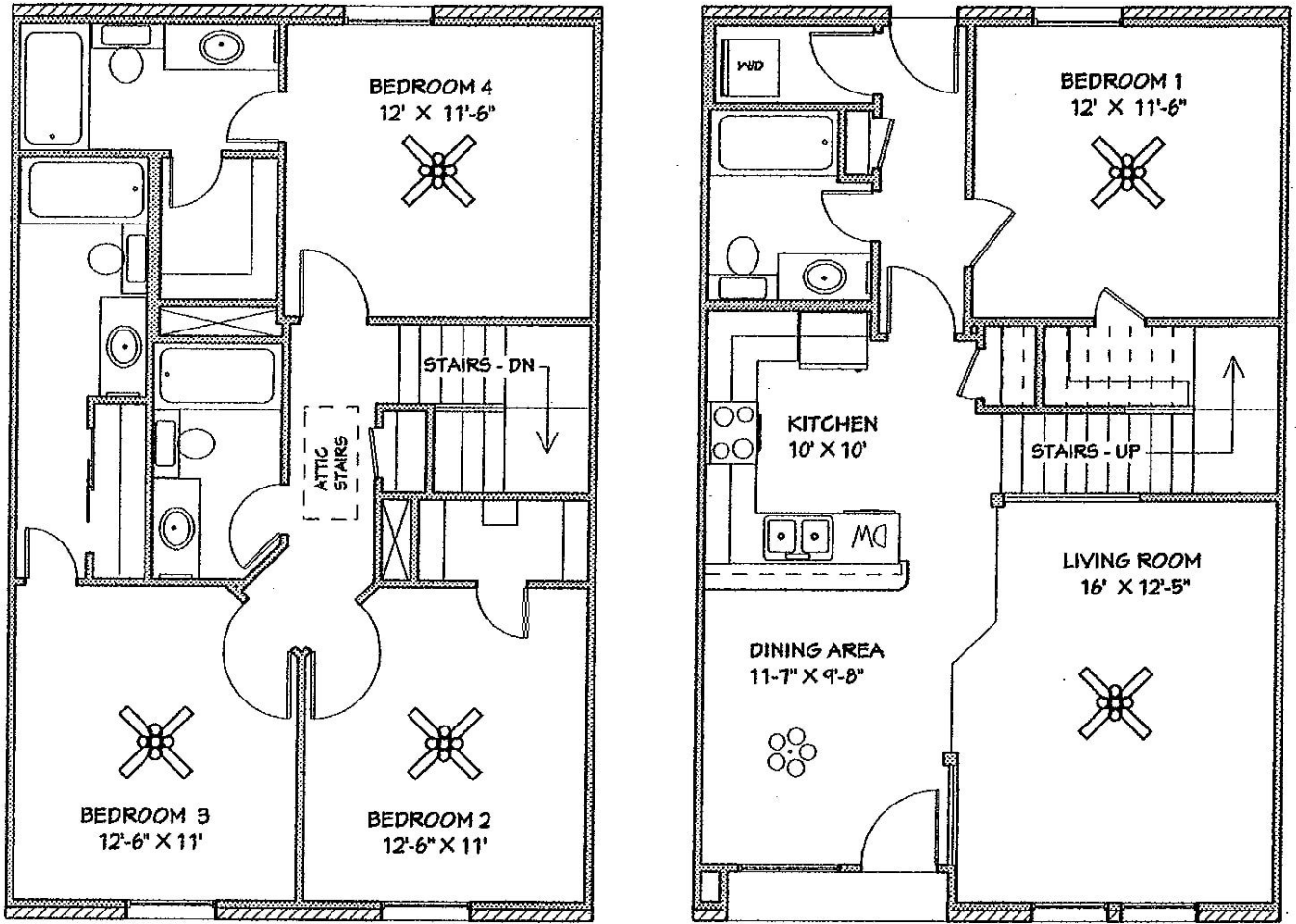
PLAN 1654 / 4 BDRM - 4 BATH / 1654 SQFT OF LIVING AREA
